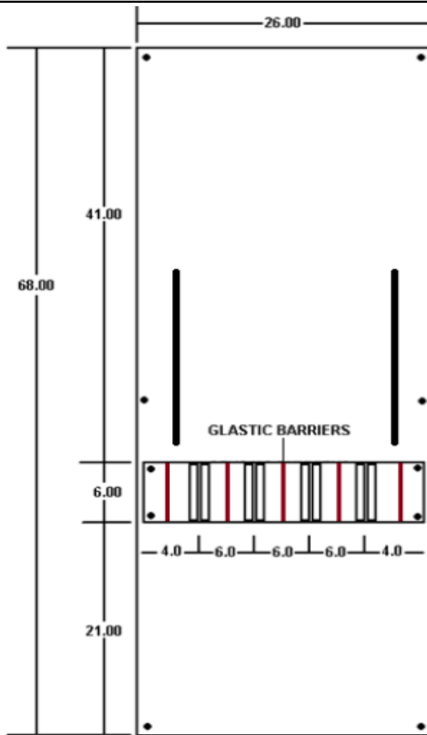
FRONT VIEW
